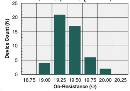
Typical On-Resistance Distribution (N=50, I_F=2mA , I_L=120mA )
