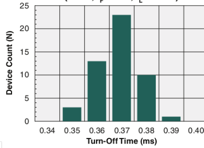
Typical Turn-Off Time (N=50, I_F=5mA , I_L=60mA )
