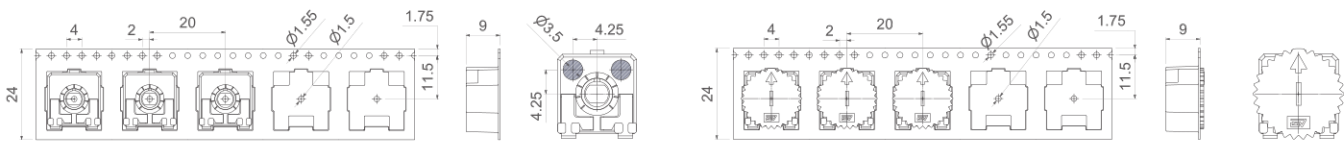
13" Reel
