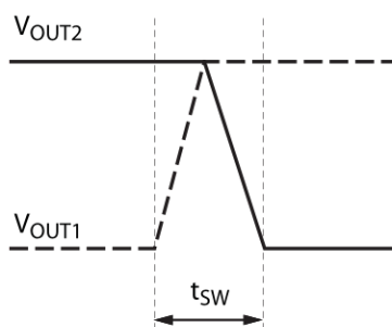
Figure 1. A1448 output soft switching with a 30 \Omega resistive load
