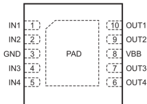
Terminal Diagram
