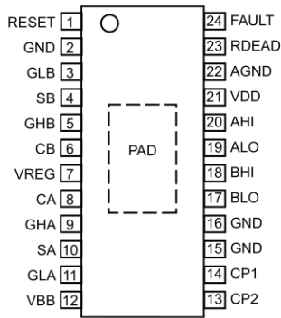
Pin-out Diagram
