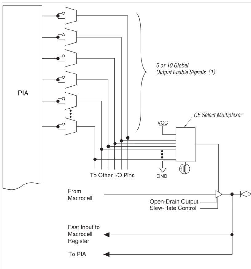
Figure 6. I/O Control Block of MAX 7000A Devices
