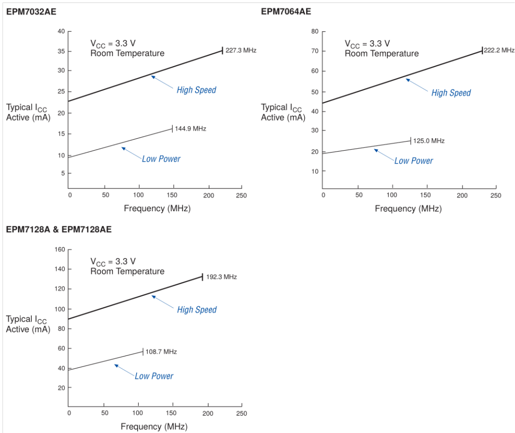
Figure 13. I_{CC} vs. Frequency for MAX 7000A Devices (Part 1 of 2)
