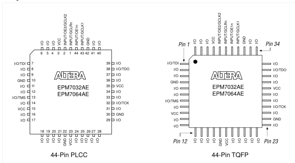
Figure 14. 44-Pin PLCC/TQFP Package Pin-Out Diagram
