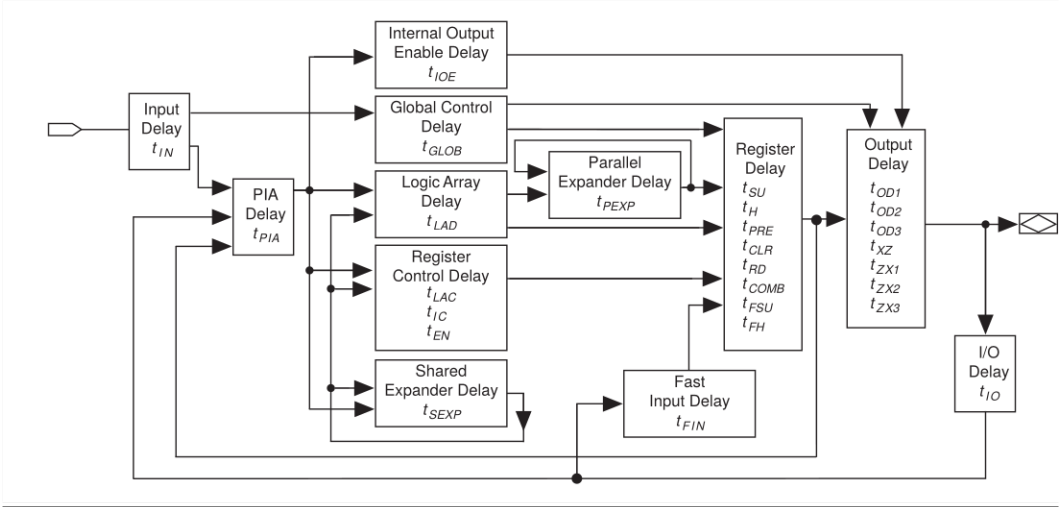
Figure 11. MAX 7000A Timing Model
