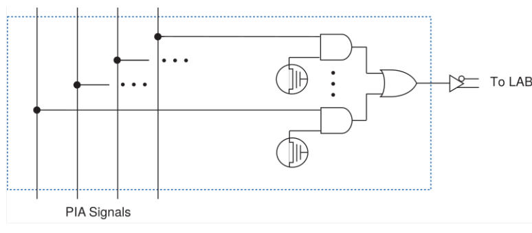
Figure 5. MAX 7000A PIA Routing
