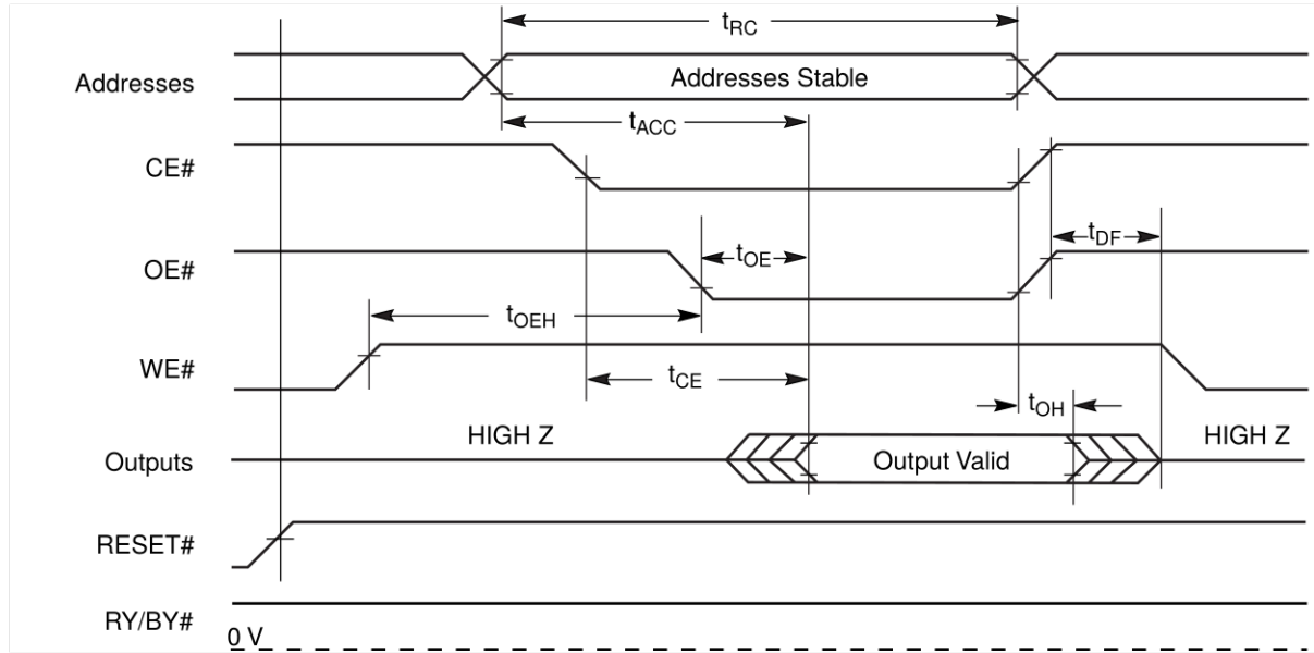
Figure 13. Read Operations Timings
