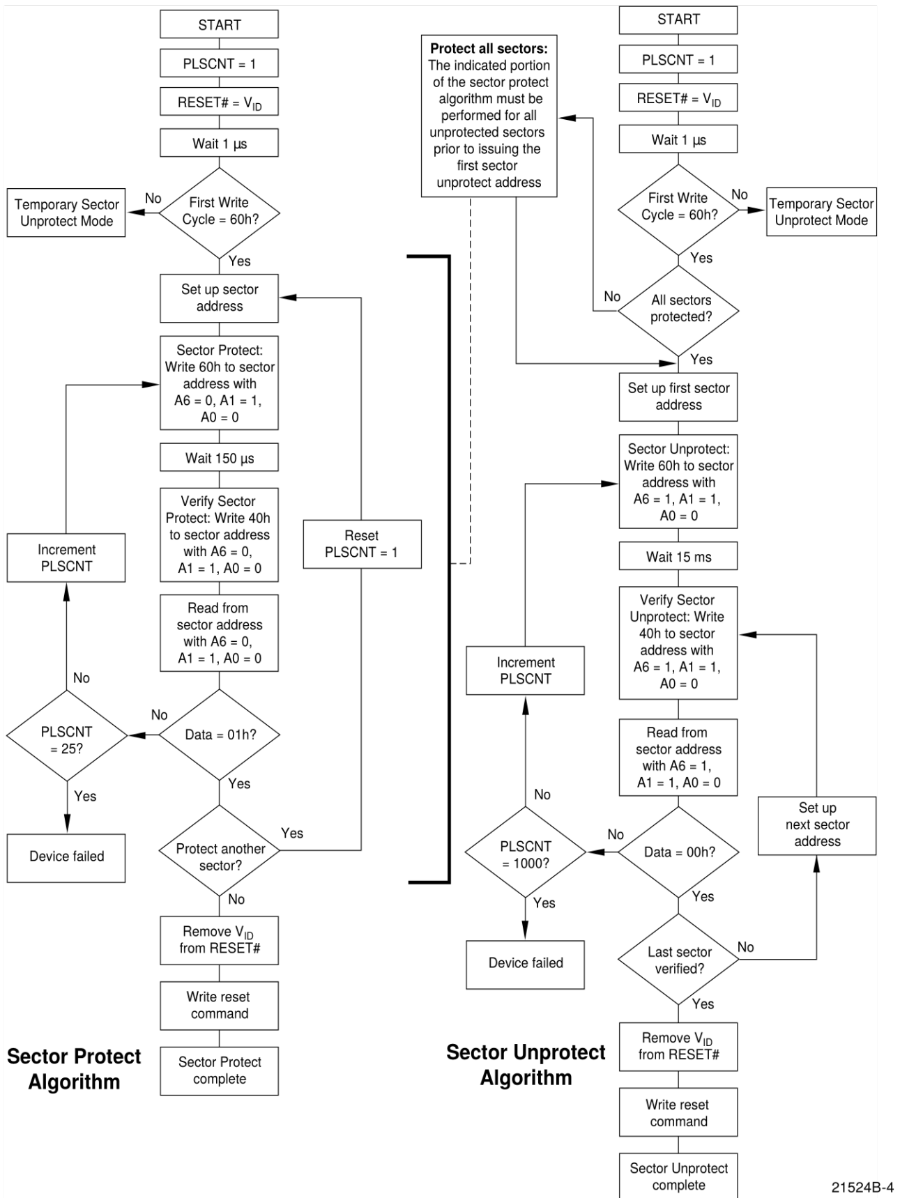
Figure 1. In-System Sector Protect/Unprotect Algorithms
