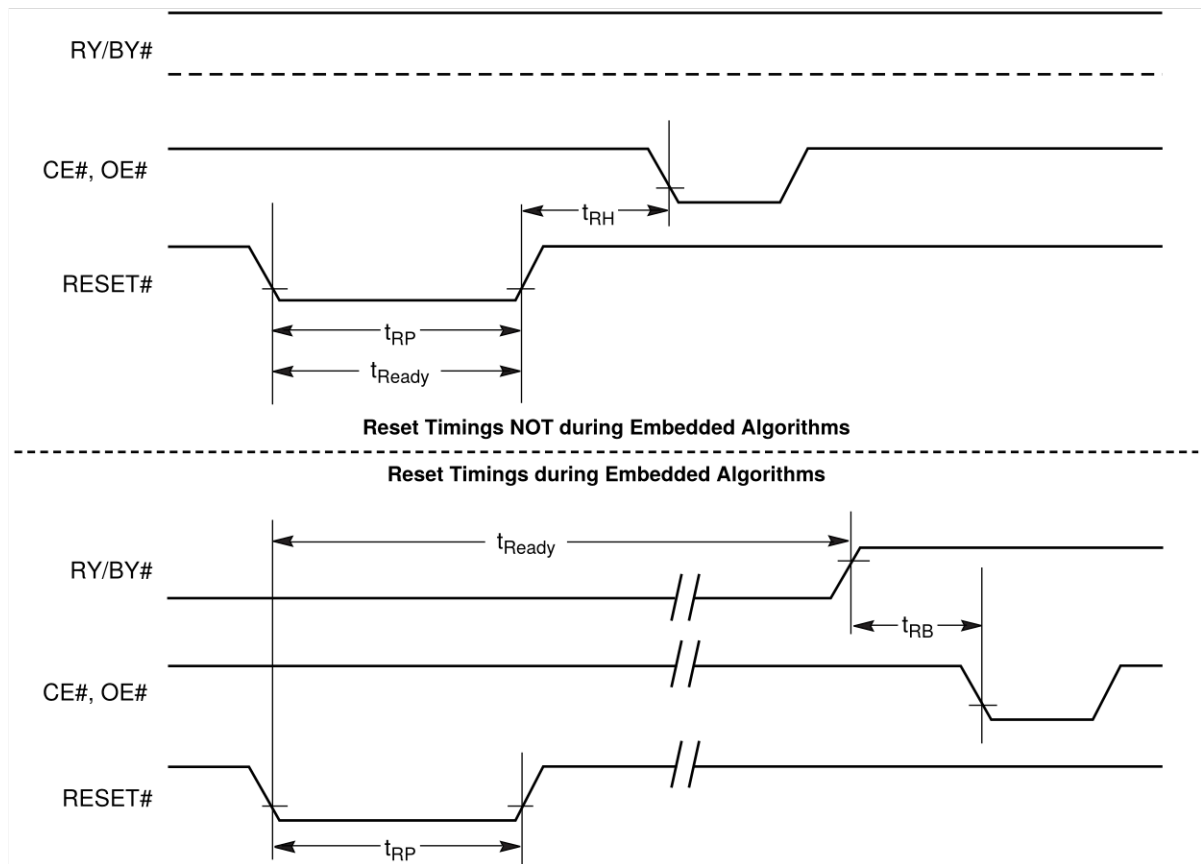
Figure 14. RESET# Timings
