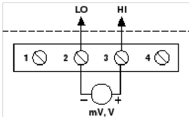
Figure 3 5B40 & 5B41 Input Field Connections
