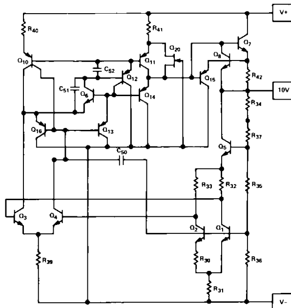
Figure 3. Simplified Schematic
