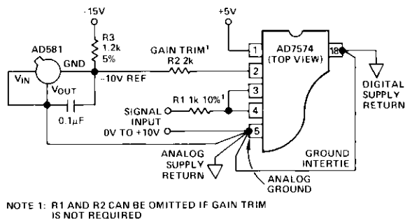
Figure 14. AD581 as Negative 10-Volt Reference for CMOS ADC
