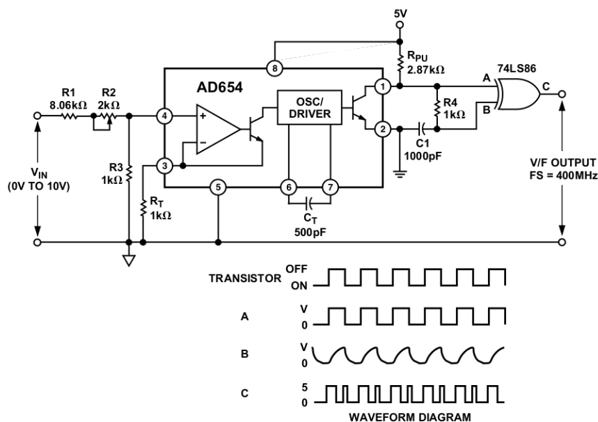
Figure 12. Frequency Doubler
