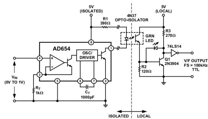
Figure 9. Optoisolator Interface
