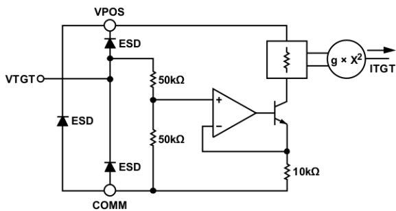
Figure 42. VTGT Interface Simplified Schematic
