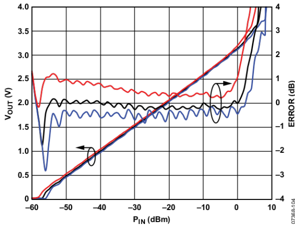
Figure 4. V_{OUT} and Log Conformance Error with Respect to 25^\circ\text{C} Ideal Line over Temperature vs. Input Amplitude at 900 MHz, CW, Typical Device
