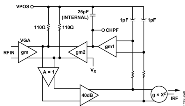
Figure 48. Offset Compensation Circuit
