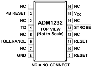
Figure 3. RW-16 Pin Configuration
