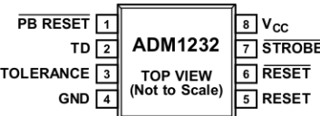
Figure 5. N-8 and R-8 Pin Configuration
