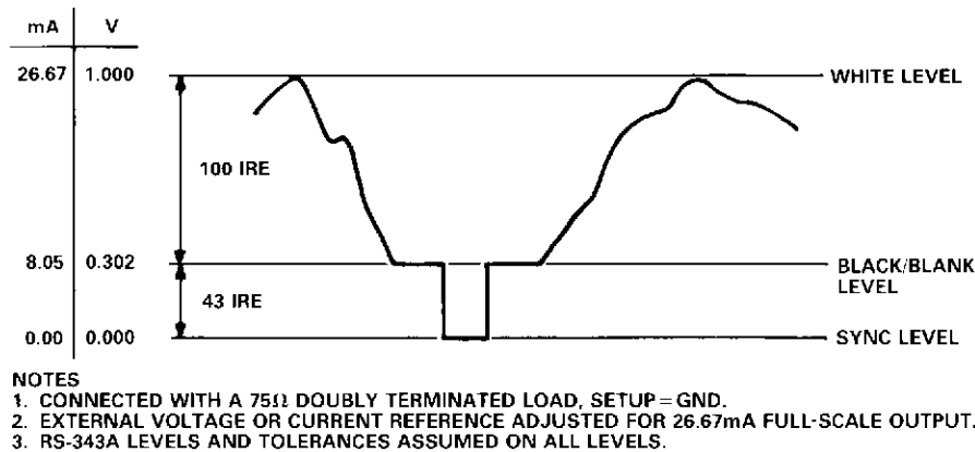
Figure 4. Composite Video Output Waveform ( \overline{\text{SETUP}} = \text{GND} )
