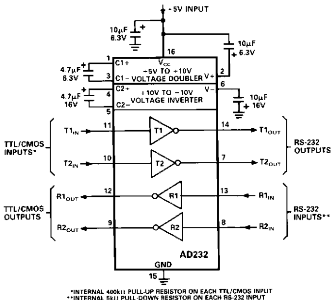
Figure 6. AD232 Typical Operating Circuit
