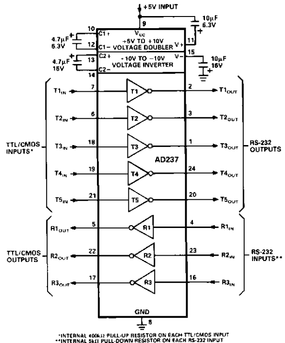
Figure 16. AD237 Typical Operating Circuit
