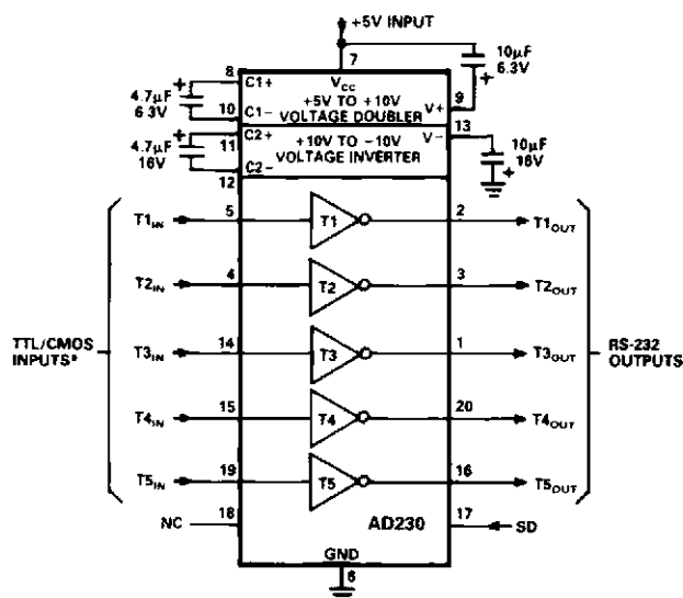
Figure 2. AD230 Typical Operating Circuit
