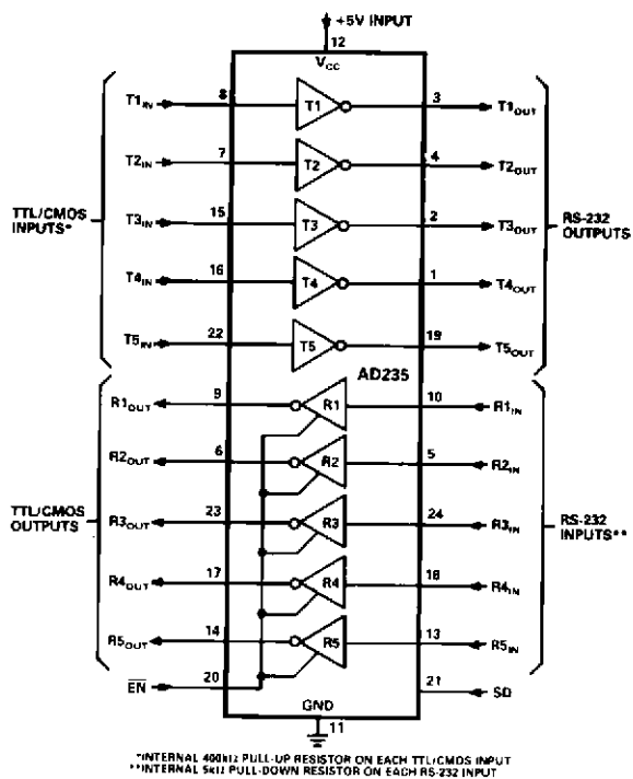
Figure 12. AD235 Typical Operating Circuit
