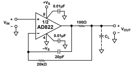
Figure 46. Extending Unity Gain Follower Capacitive Load Capability Beyond 350 pF
