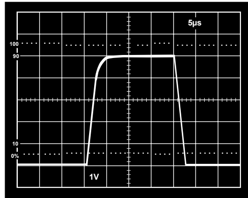
Figure 48. Pulse Response of In-Amp to a 500 mV p-p Input Signal; V_S
