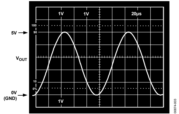
Figure 3. Gain-of-2 Amplifier; V_S = 5, 0 , V_{IN} = 2.5\text{ V} Sine Centered at 1.25\text{ V} , R_L = 100\ \Omega
