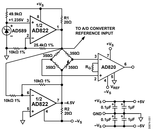
Figure 51. Low Dropout Bipolar Bridge Driver
