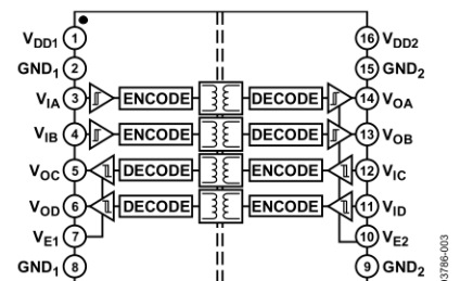
Figure 3. ADuM1402 Functional Block Diagram
