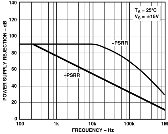
TPC 21. Power Supply Rejection vs. Frequency @ ±15 V
