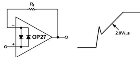
Figure 37. Pulsed Operation
