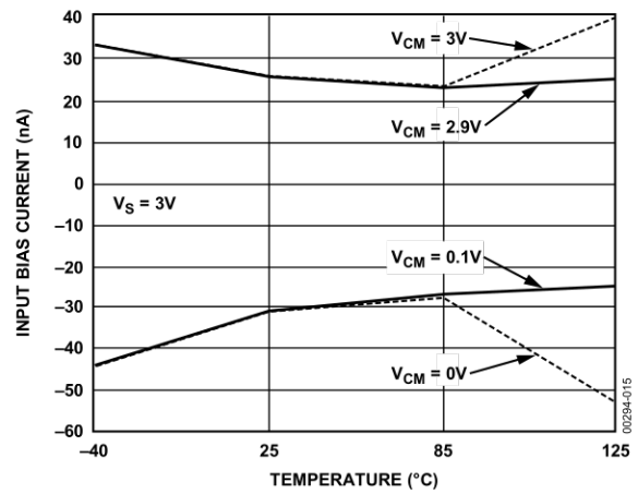
Figure 10. Input Bias Current vs. Temperature, V_S = 3V
