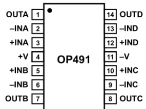
Figure 3. 14-Lead Narrow-Body SOIC
