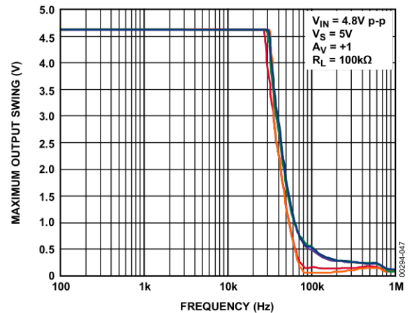
Figure 42. Maximum Output Swing vs. Frequency, V_S = 5\text{ V}
