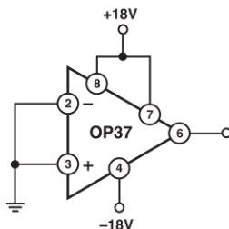
Figure 3. Burn-In Circuit
