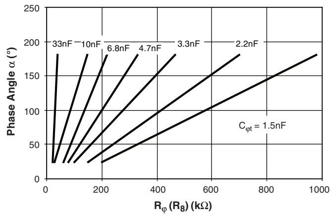
Figure 7-1. Ramp Control
