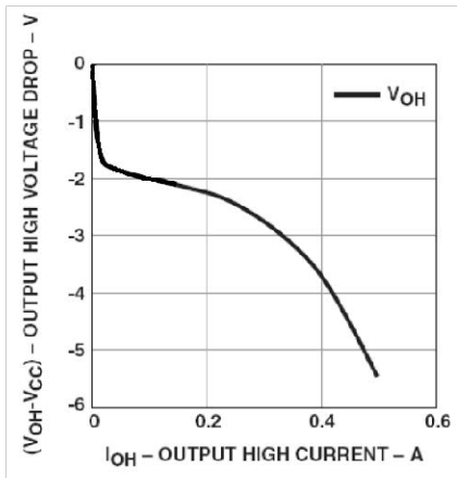
Figure 9: V_{OH} vs. I_{OH}
