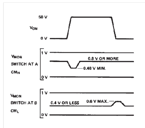
Figure 11. Typical Waveforms for Common Mode Transient Immunity.
