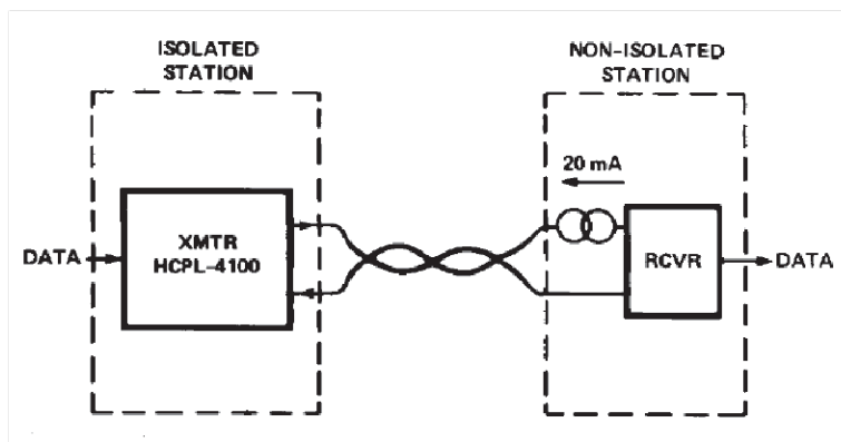
Figure 12. Simplex Point to Point Current Loop System Configuration.
