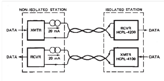
Figure 16. Full Duplex Point to Point Current Loop System Configuration.
