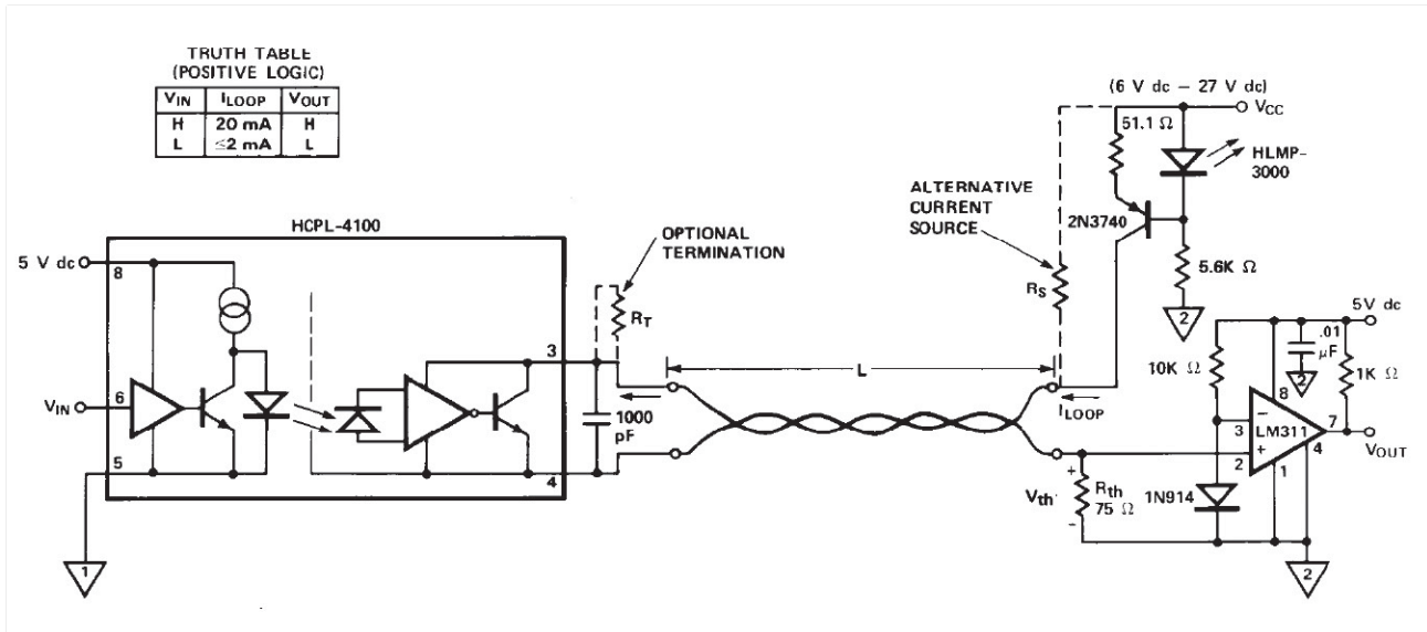
Figure 13. Recommended Non-Isolated Active Receiver with HCPL-4100 Isolated Transmitter for Simplex Point to Point 20 mA Current Loop.
