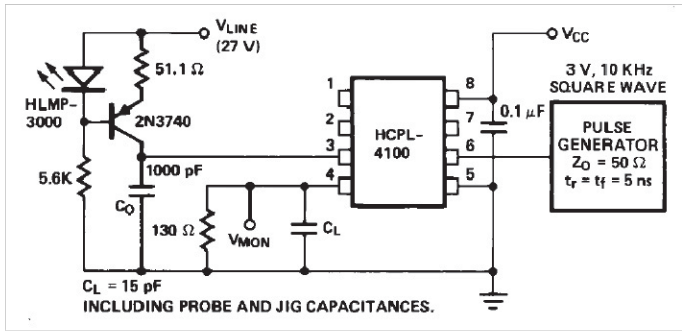
Figure 6. Test Circuit for t_{PLH} , t_{PHL} , t_r and t_f .
