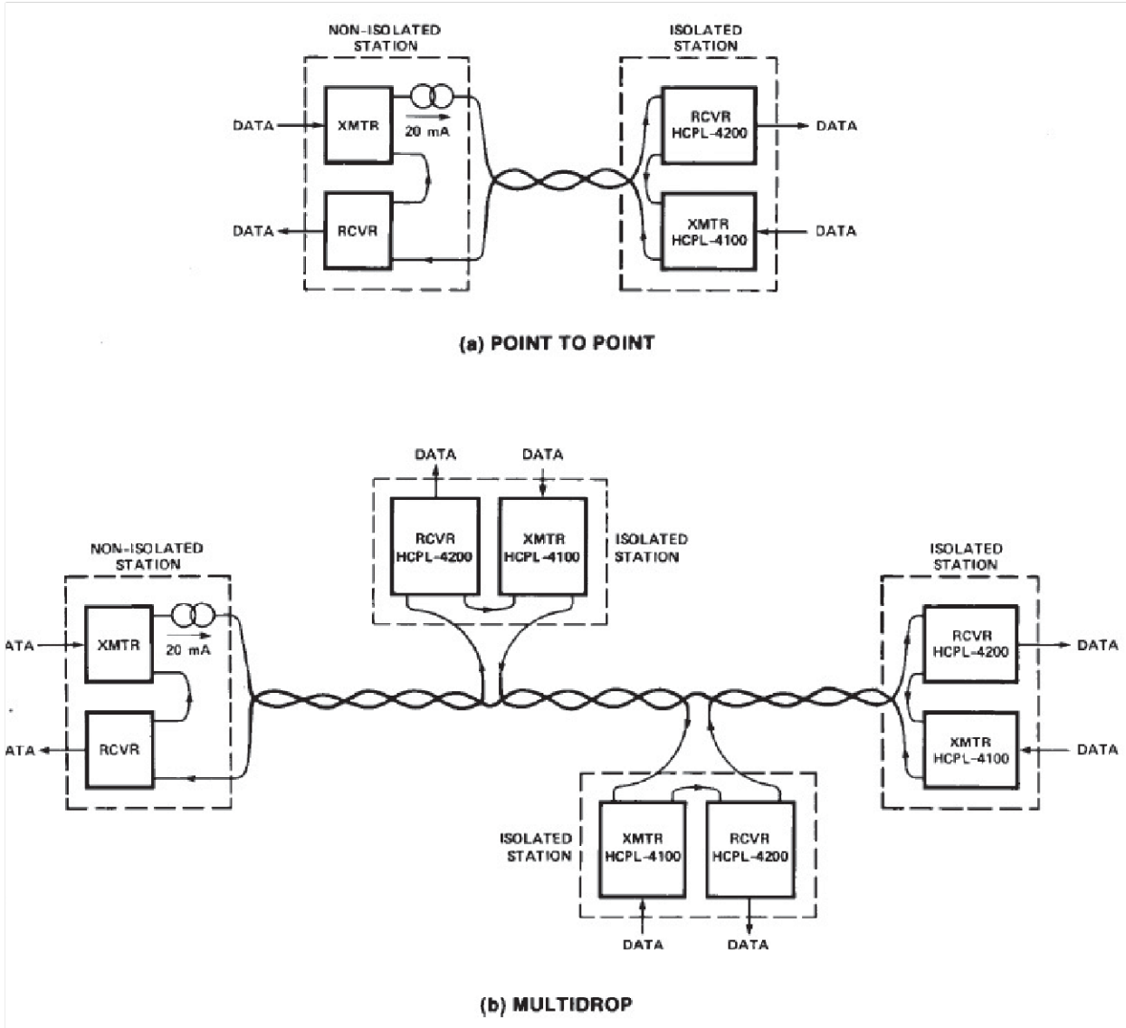
Figure 17. Half Duplex Current Loop System Configurations for (a) Point to Point, (b) Multidrop.
