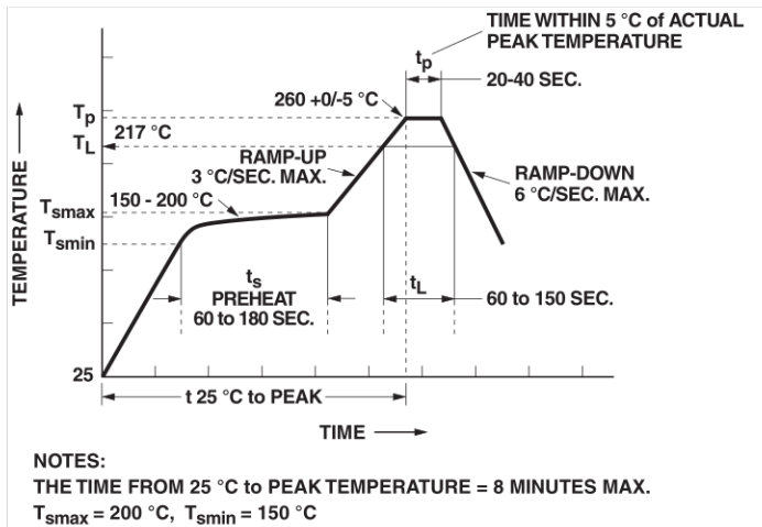
Figure 2. Pb-Free IR Profile.
