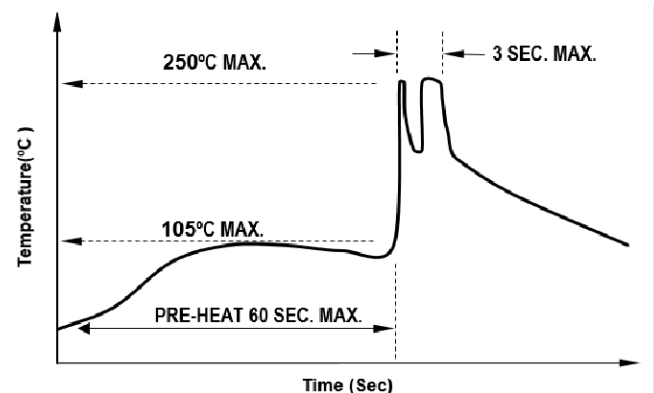
Figure 17: Recommended Wave Soldering Profile
