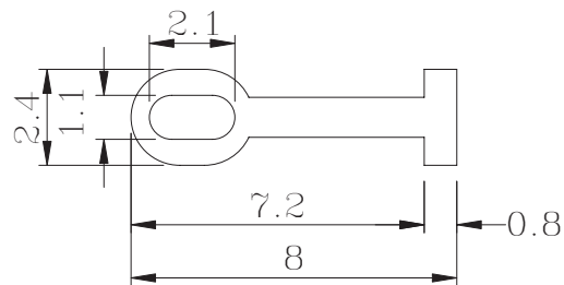
TERMINAL DETAIL SCALE: 5/1
