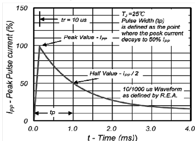
Fig 2: Pulse Waveform
