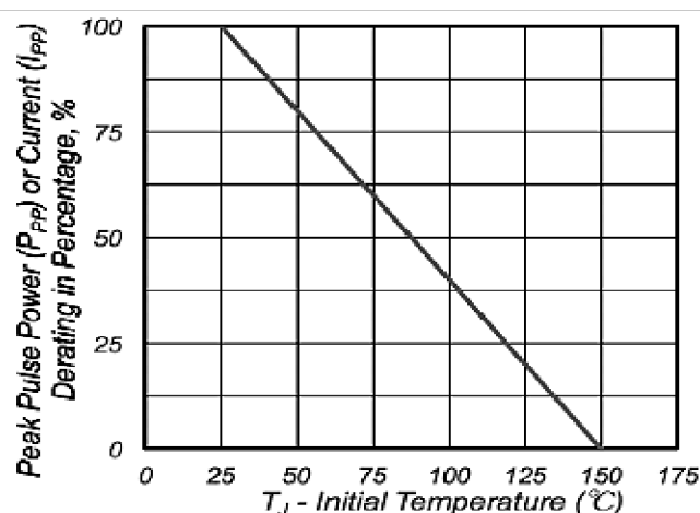
Fig 3: Pulse Derating Curves
