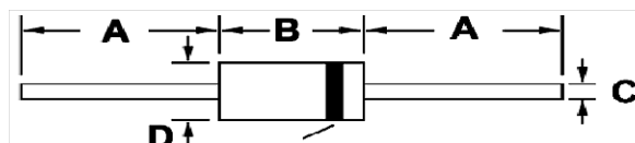
DO-201AD Axial Leaded Plastic Package
