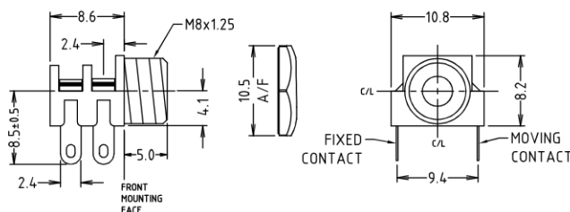
S6/BB mono switched 3.5mm Jack Socket. Panel mounting with solder tags. Also available with Special 'C' Contact to suit Far Eastern plugs.
