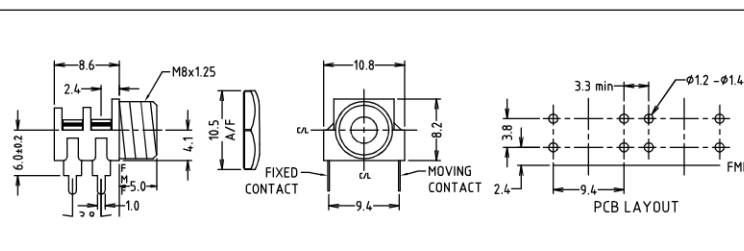
S6/BB PC mono switched 3.5mm Jack Socket. Right angle PCB mounting. Also available with Special 'C' Contact to suit Far Eastern plugs.
