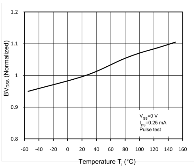
Figure 5. Normalized BV DS(sat) vs. Temperature
