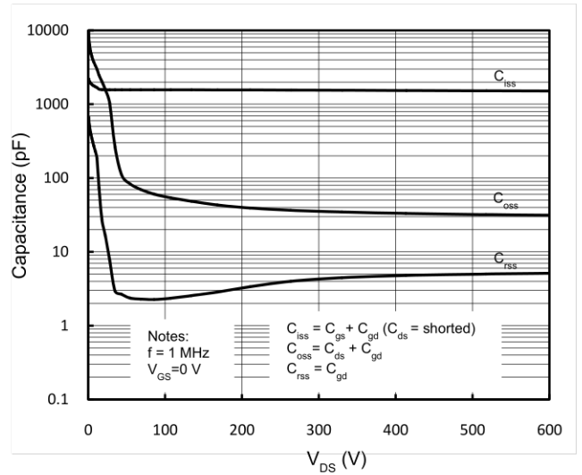
Figure 8. Capacitance Characteristics
