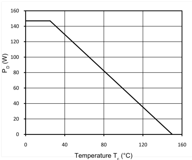
Figure 9. Power Dissipation
