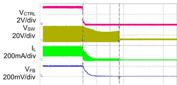
Shutdown PWM Dimming Duty=100%
