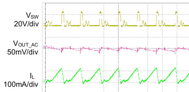
Steady State PWM Dimming Duty=25%
