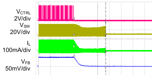
Shutdown PWM Dimming Duty=25%
