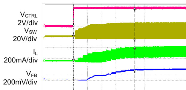
Start up PWM Dimming Duty=100%
