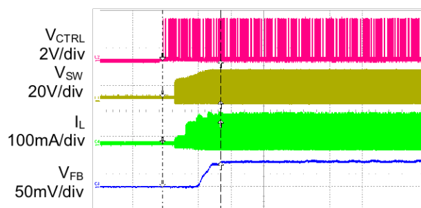
Start up PWM Dimming Duty=25%
