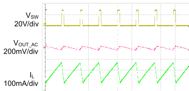
Steady State PWM Dimming Duty=100%
