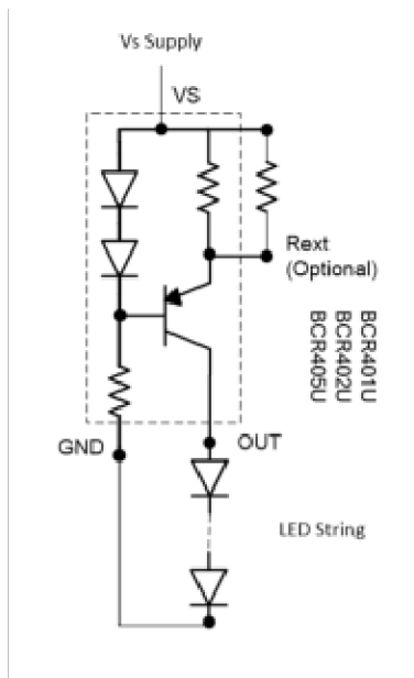
Figure: 1 Typical Application Circuit for BCR40X LED Driver
