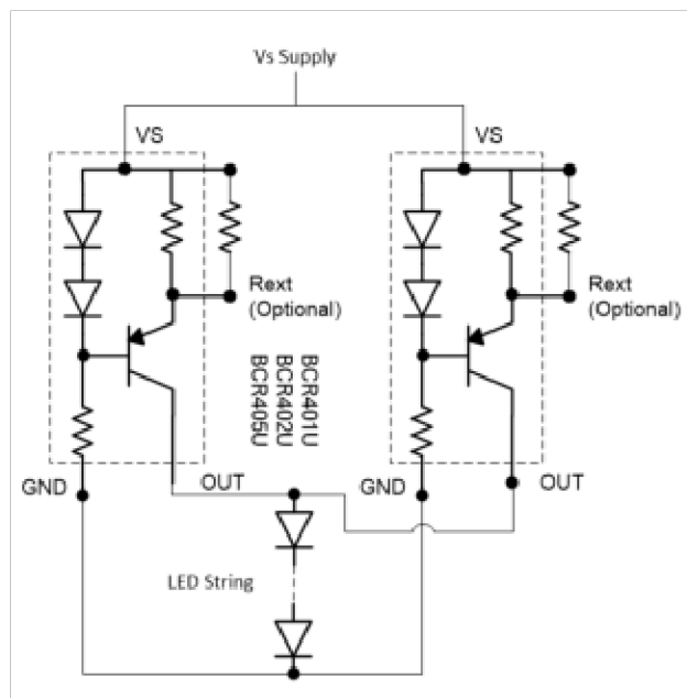
Figure: 2 Application Circuit for Increasing LED Current
