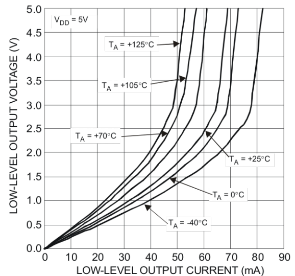
Figure 12 Low-Level Output Voltage vs. Low-Level Output Current
