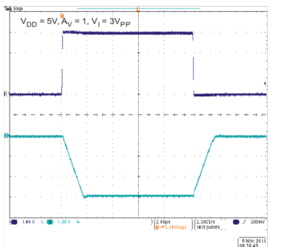
Figure 24 Inverting Large Signal Pulse Response V_{DD} = 5V
