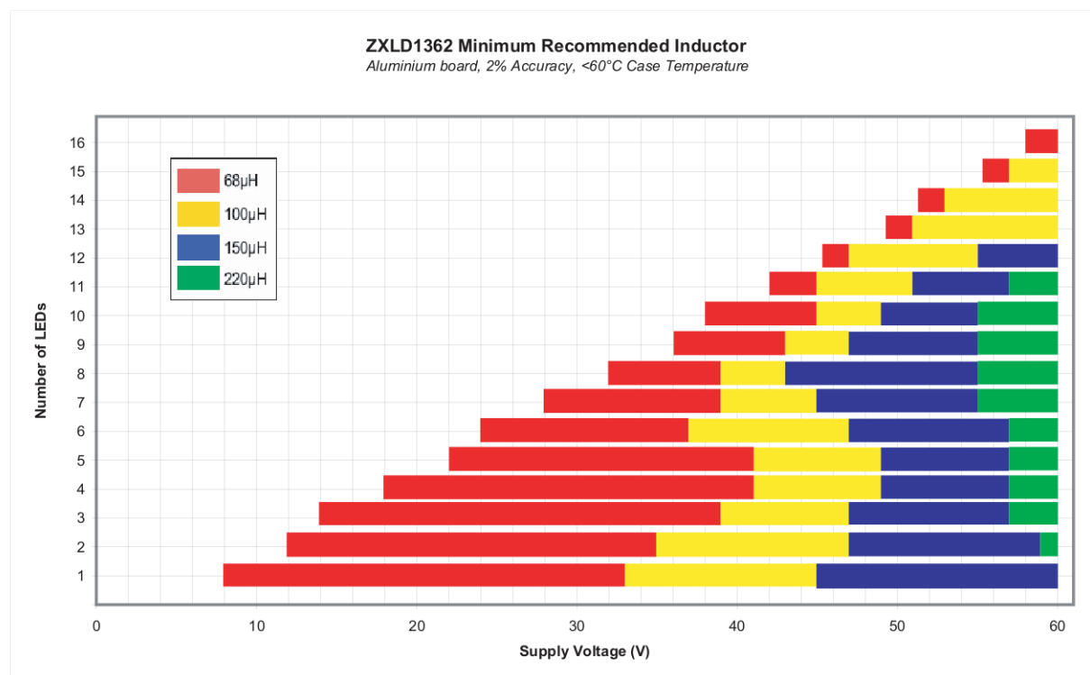
Figure 3 ZXLD1362 Minimum recommended Inductor
