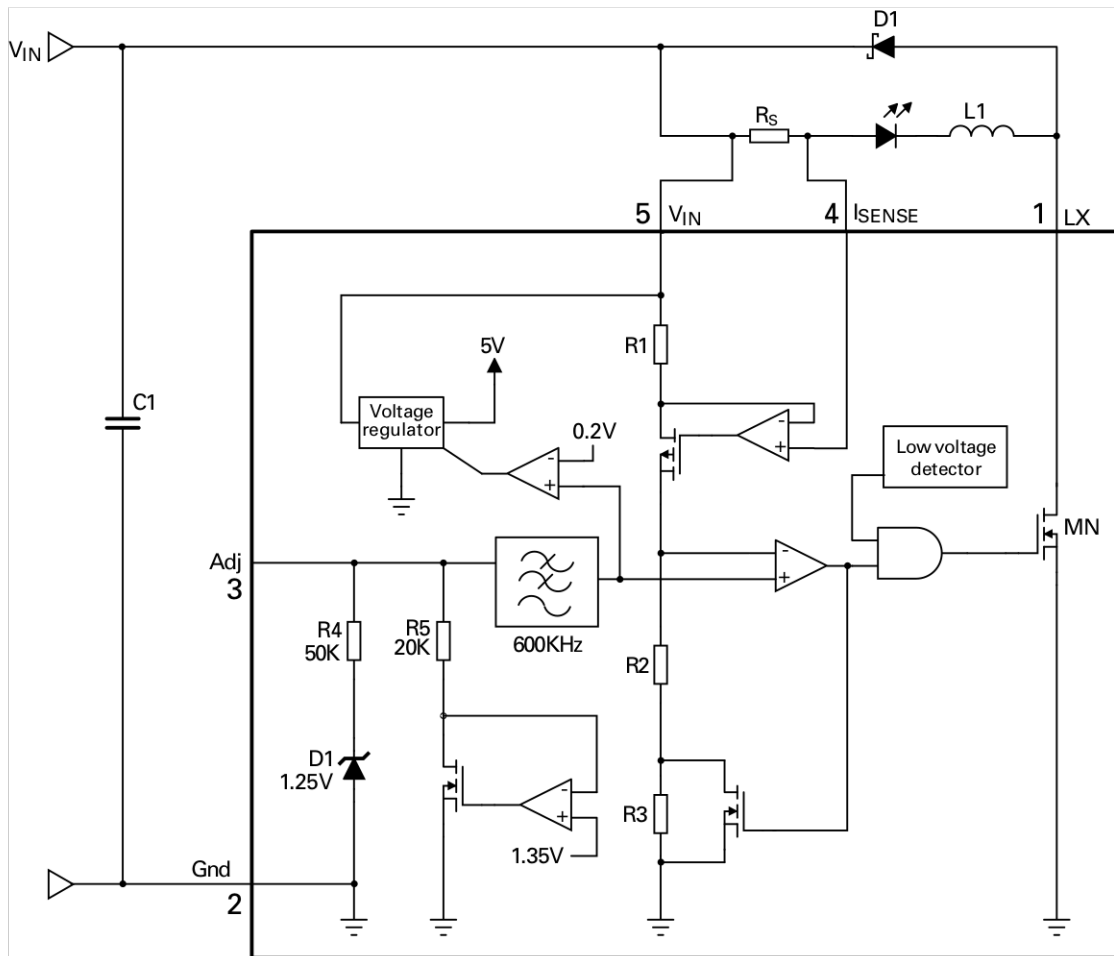
Figure 1 Block diagram
