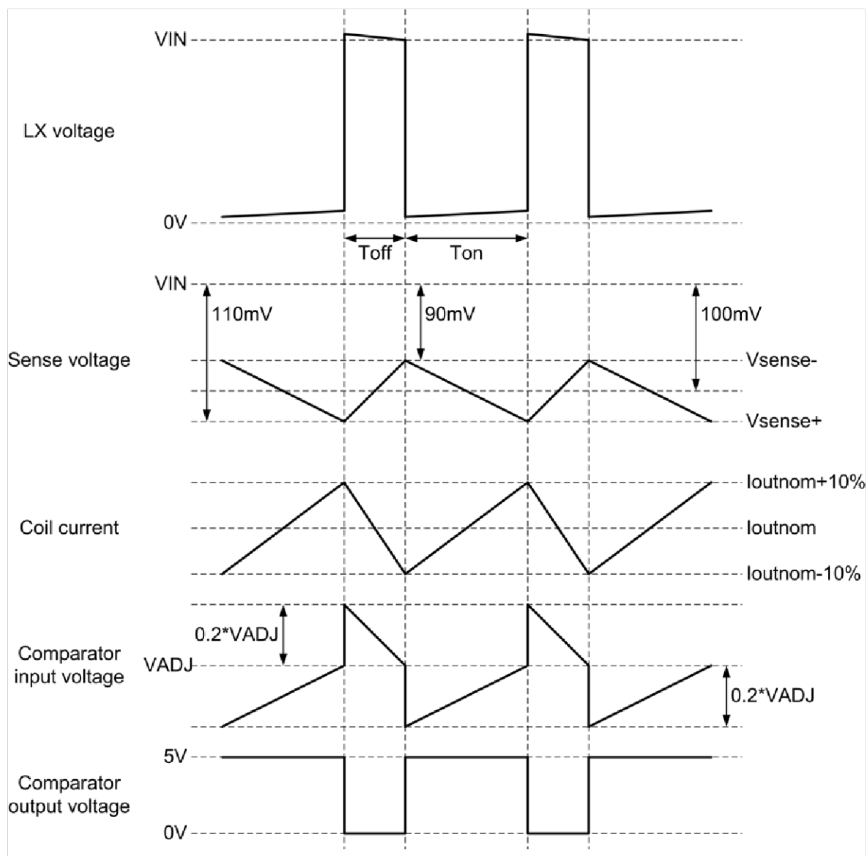
Figure 2 Theoretical operating waveforms
