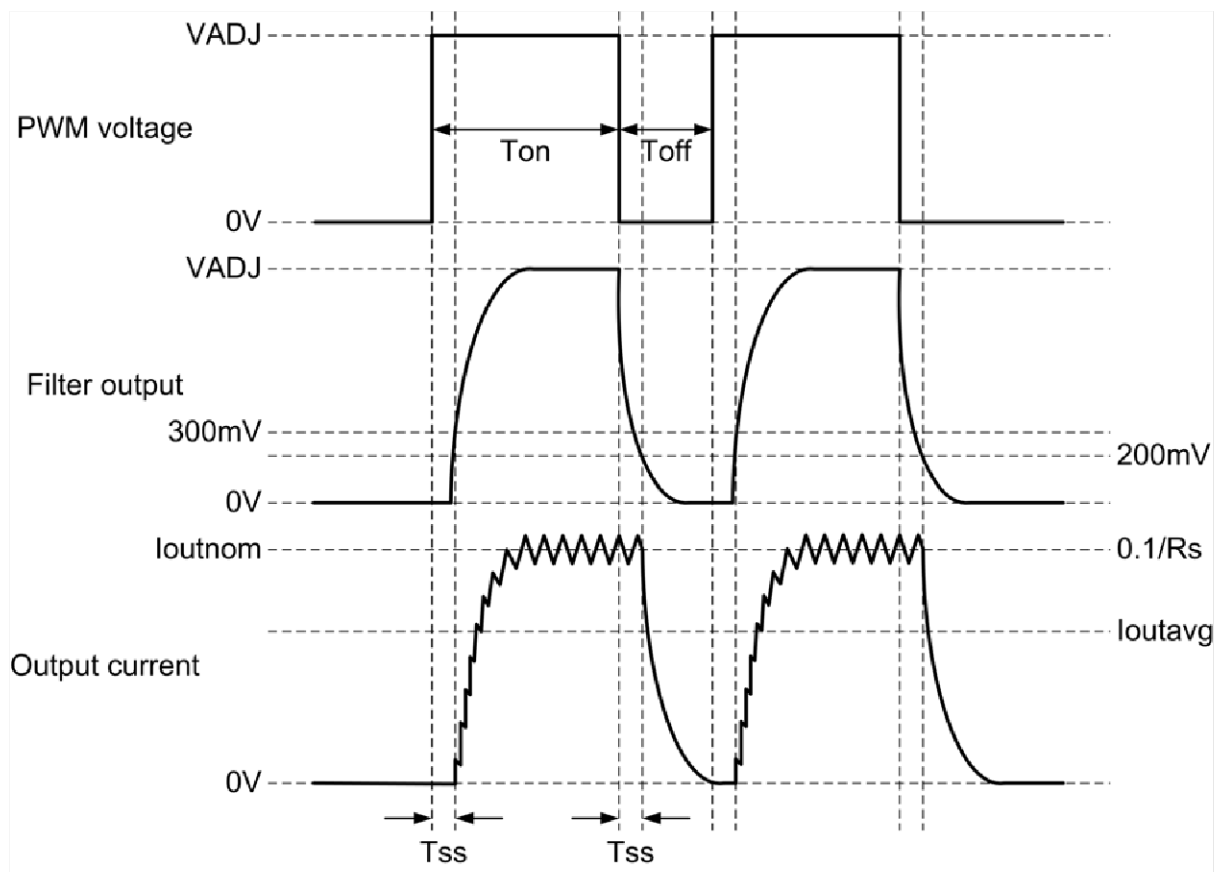
Figure 4 Low frequency PWM operating waveforms
