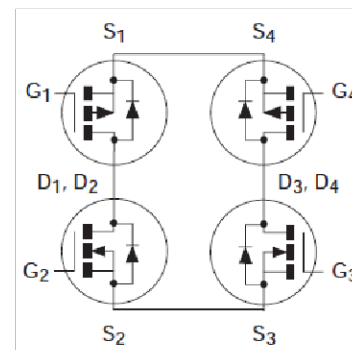
Internal Schematic
