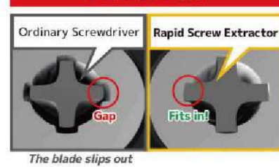
Innovative design of the blade tip
