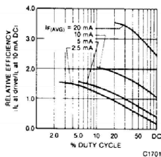
Fig. 11. Relative Efficiency vs. Duty Cycle
