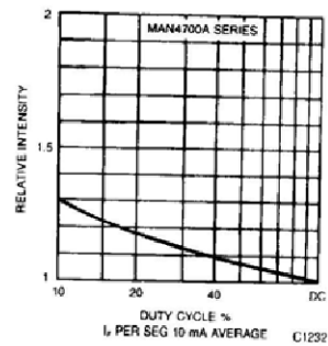
Fig. 14. Luminous Intensity vs. Duty Cycle
