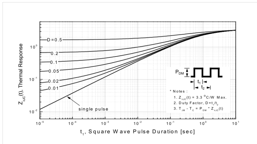
Figure 11-2. Transient Thermal Response Curve for FDPF15N65
