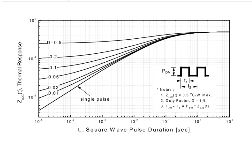
Figure 11-1. Transient Thermal Response Curve for FDP15N65
