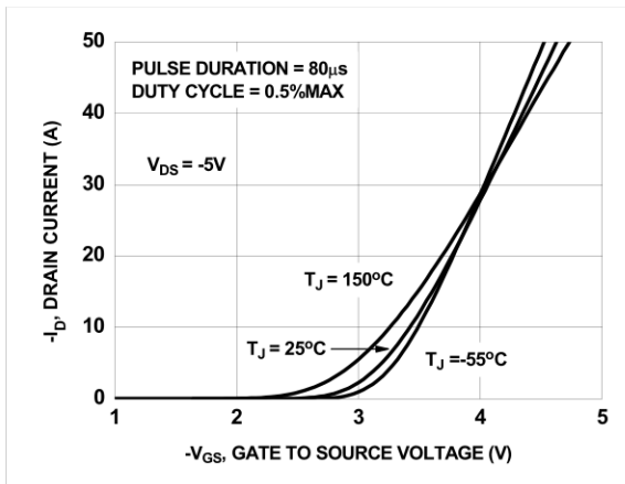
Figure 5. Transfer Characteristics
