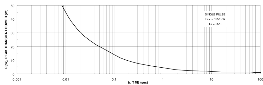
11. Single Pulse Maximum Power Dissipation.
