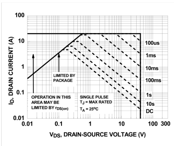
Figure 11. Forward Bias Safe Operating Area
