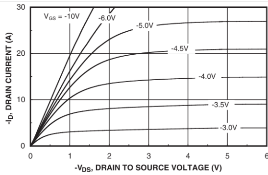
Figure 11. On-Region Characteristics.
