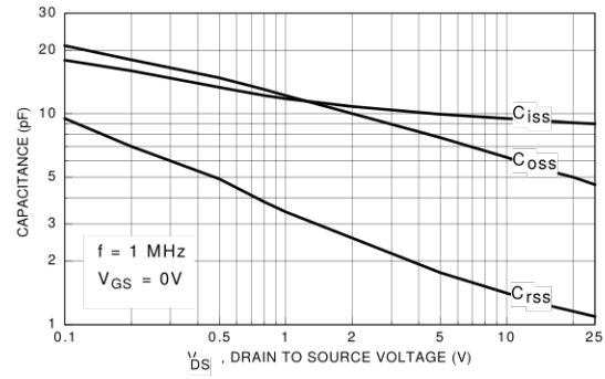
Figure 8. Capacitance Characteristics.
