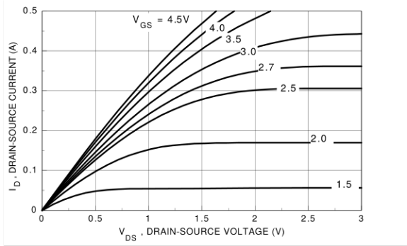
Figure 1. On-Region Characteristics.
