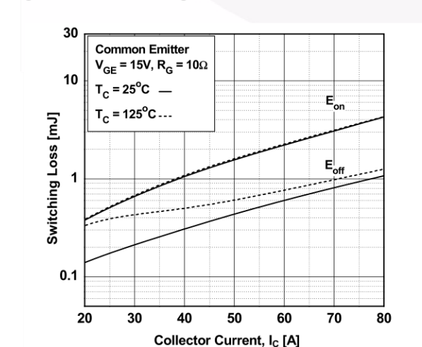
Figure 17. Switching Loss vs. Collector Current
