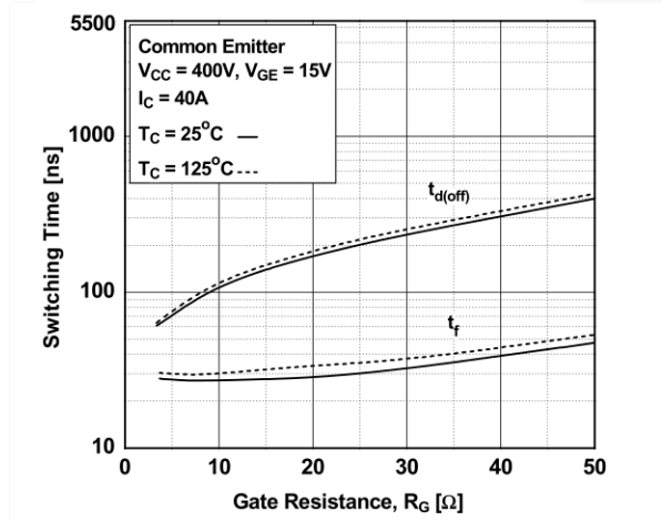
Figure 13. Turn-off Characteristics vs. Gate Resistance
