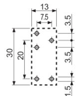
95.13.2 Copper side view
