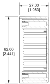
SECTION B-B
