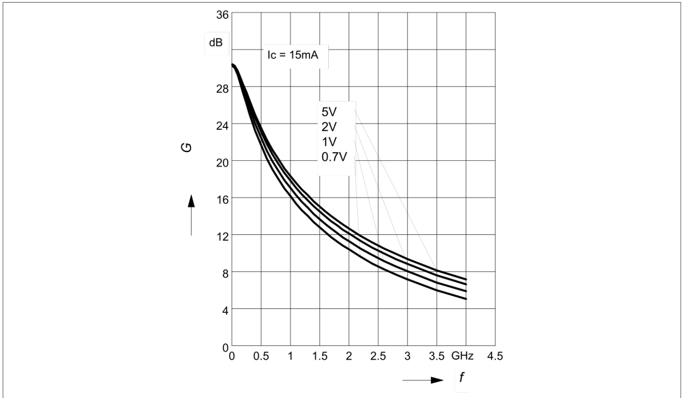
Figure 6 Transducer Gain IS_{21}I^2 = f(f), I_C = 15 mA, V_{CE} = parameter
