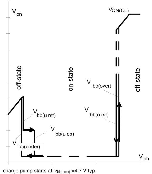
Figure 7a: Overvoltage:
