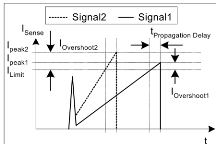
Figure 19 Current Limiting
