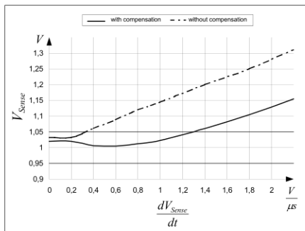
Figure 20 Overcurrent Shutdown
