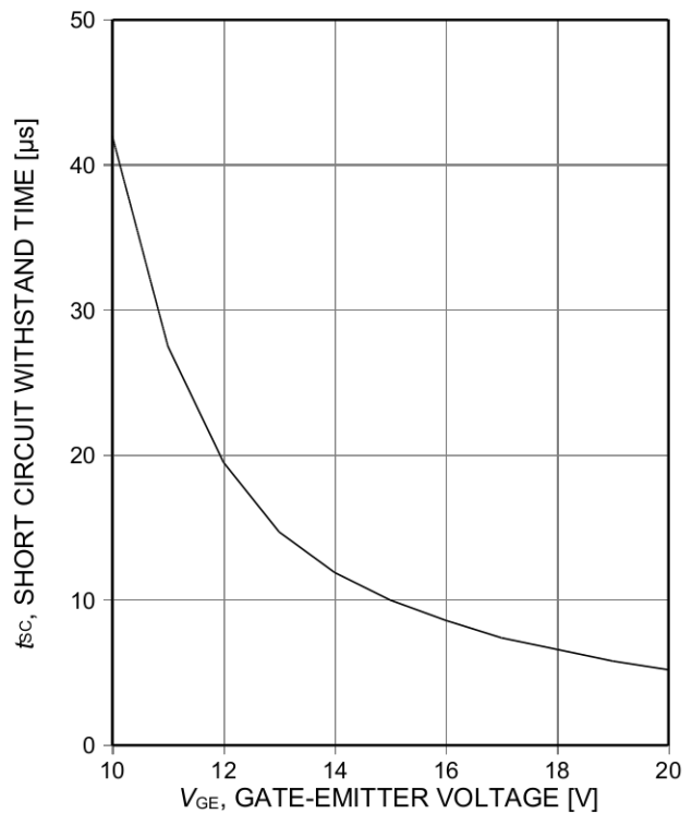
Figure 20. Short circuit withstand time as a function of gate-emitter voltage ( V_{CE} \le 600V , start at T_j \le 150^\circ C )
