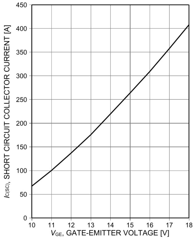
Figure 18. Typical short circuit collector current as a function of gate-emitter voltage ( V_{CE} \leq 600V , T_{vj} \leq 75^{\circ}C )
