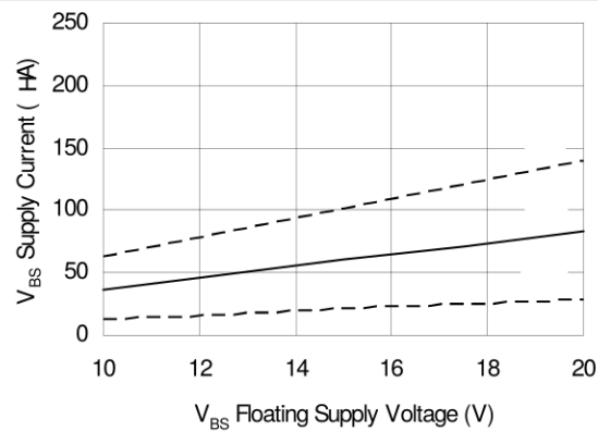
Figure 17B. V_{BS} Supply Current vs. V_{BS} Floating Supply Voltage
